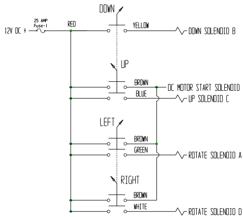
ELECTRICAL WIRING
