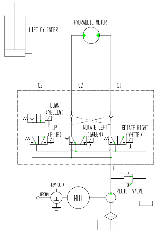
HYDRAULIC SCHEMATIC
