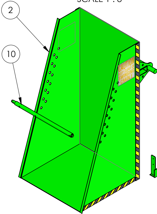
DETAIL A SCALE 1 : 8
